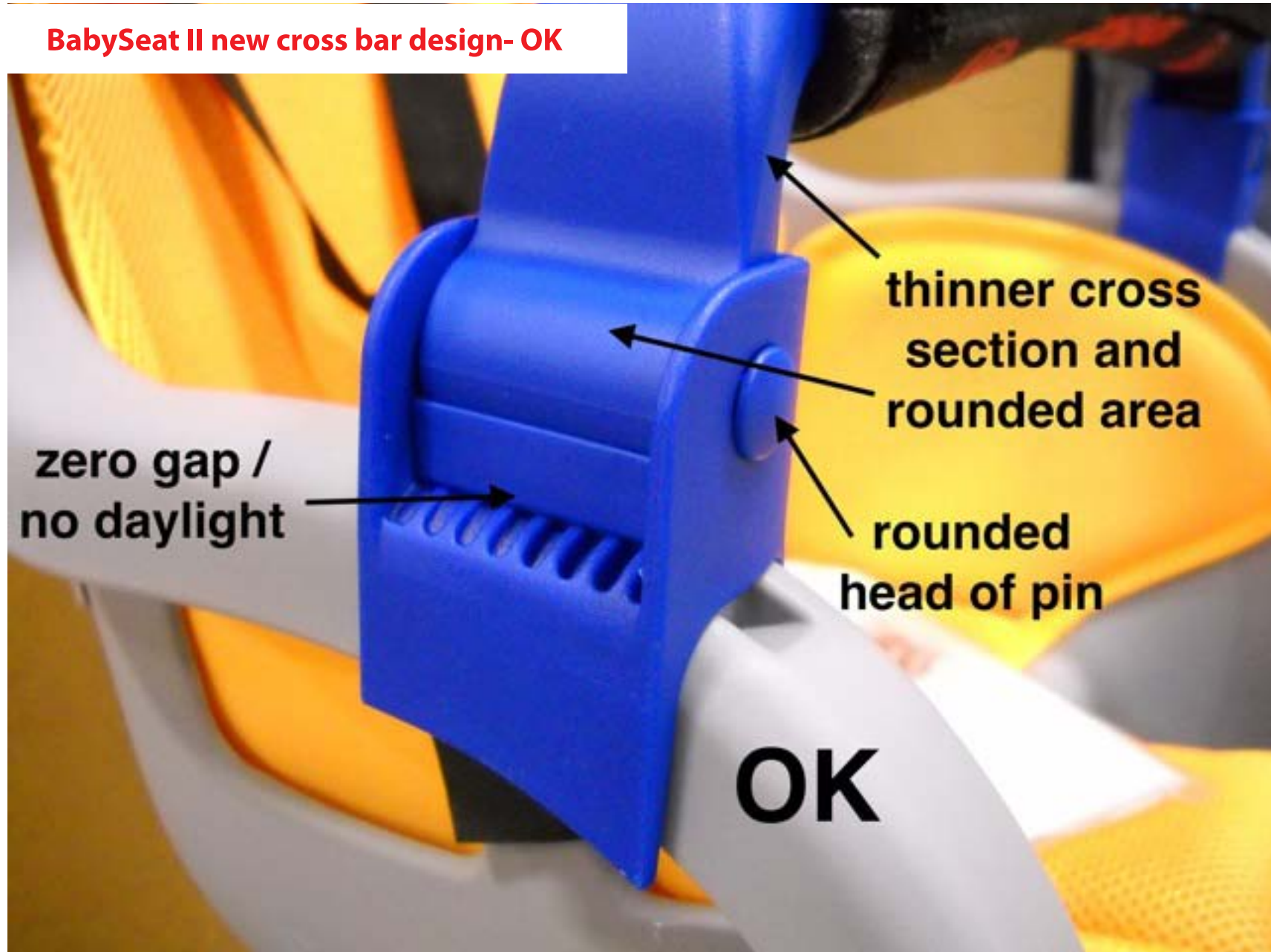
BabySeat II new cross bar design- OK
